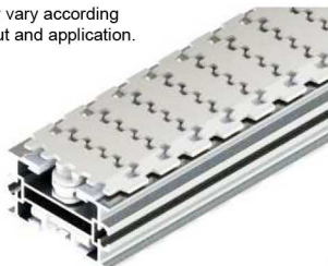
Chain Width 140mm
